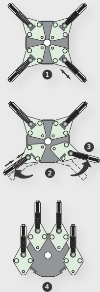
Crane bookfold mechanism
